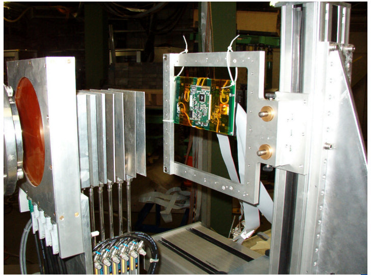
Electronics under proton test
