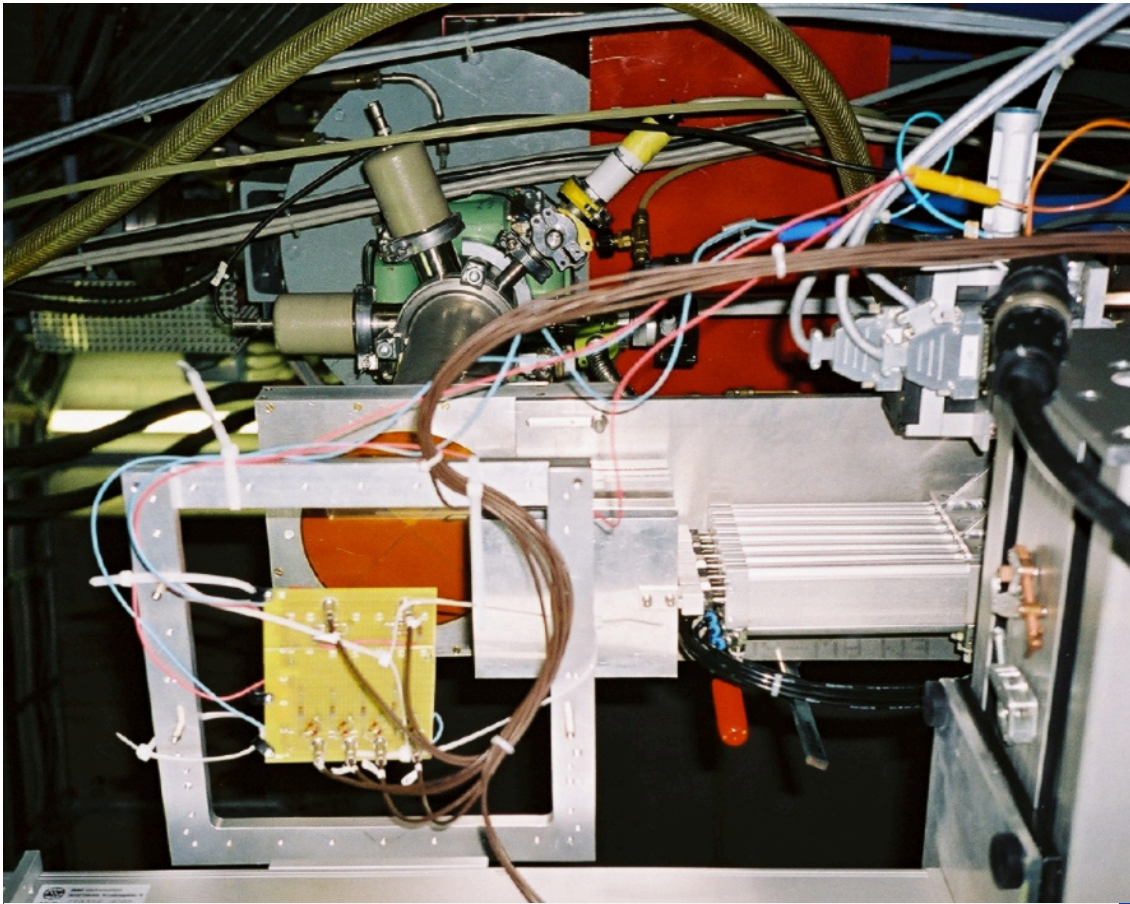
Test setup of MOSFETs in proton beam
