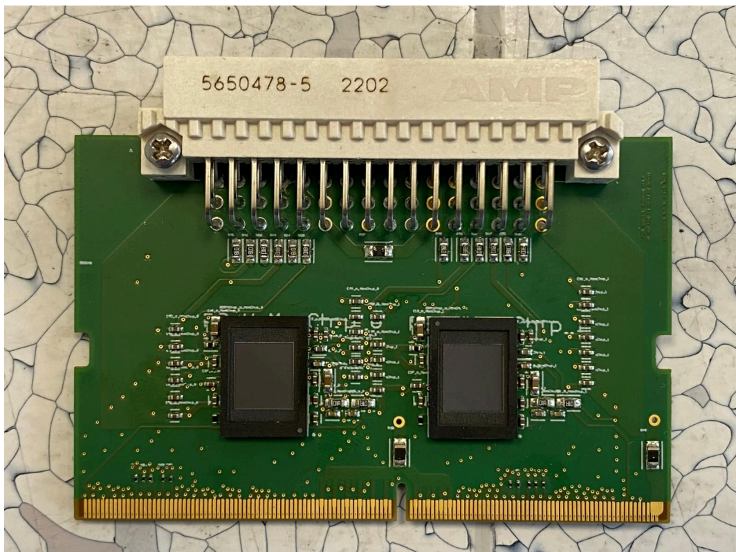
Thinned chips for heavy ion tests assembled on PCB
